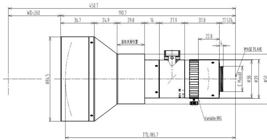
SNT1IR027W260C-L
