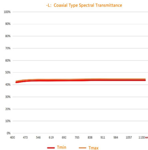
SNT1IR027W260C-L
